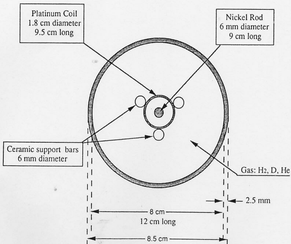
Fig. 1. - Cross-section of our experimental set-up.
