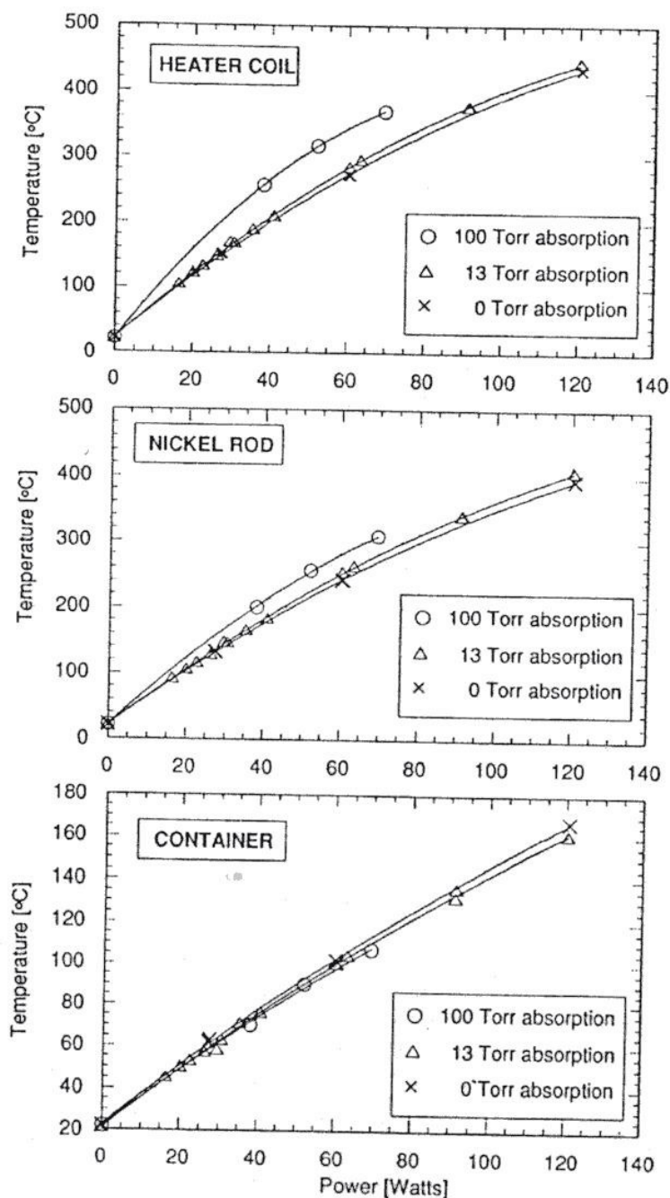
Fig. 4. - Coil, rod and container temperature vs. input power for 3 cases ( \Delta p = 0, 13 and 100 Torr); coil material is platinum.
