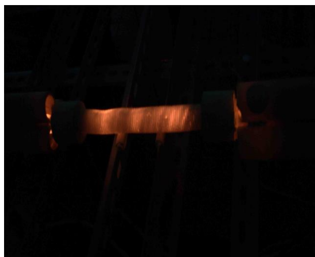
Figures 12a, 12b. E-Cat operating during the test. Note the Inconel resistors leaving the caps and entering the rods, where they are connected to the copper cables of the power supply. The resistors appear to glow intensely in the parts lying outside the caps, whereas inside the reactor body they seem to shade an underlying emission of light. This may be explained if we consider that the main source of energy inside the reactor body is actually the charge, and that it is emitting more light than the resistors. These are not visible through the caps, which are thicker than the reactor body. Upon leaving the reactor, however, the resistors emit heat almost exclusively by radiation (convection is negligible here, as they are inside the rods): there are no brighter sources of light which can “outshine” them, nor masses of alumina that can cool them. Their temperature is moreover fairly high, on account of the current they carry and the heat extracted by conduction from the reactor. Figure 12b was taken in the dark, from the opposite side to that of 12a. One of the three sets of hollow rods is visible, and another patch of insulating alumina cement on the second metal strut in the middle, added without modifying the setup.
