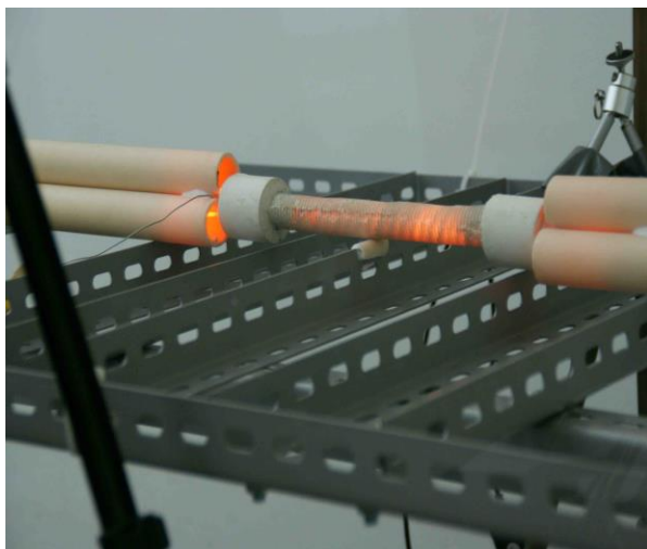
Figures 12a, 12b. E-Cat operating during the test. Note the Inconel resistors leaving the caps and entering the rods, where they are connected to the copper cables of the power supply. The resistors appear to glow intensely in the parts lying outside the caps, whereas inside the reactor body they seem to shade an underlying emission of light. This may be explained if we consider that the main source of energy inside the reactor body is actually the charge, and that it is emitting more light than the resistors. These are not visible through the caps, which are thicker than the reactor body. Upon leaving the reactor, however, the resistors emit heat almost exclusively by radiation (convection is negligible here, as they are inside the rods): there are no brighter sources of light which can “outshine” them, nor masses of alumina that can cool them. Their temperature is moreover fairly high, on account of the current they carry and the heat extracted by conduction from the reactor. Figure 12b was taken in the dark, from the opposite side to that of 12a. One of the three sets of hollow rods is visible, and another patch of insulating alumina cement on the second metal strut in the middle, added without modifying the setup.
